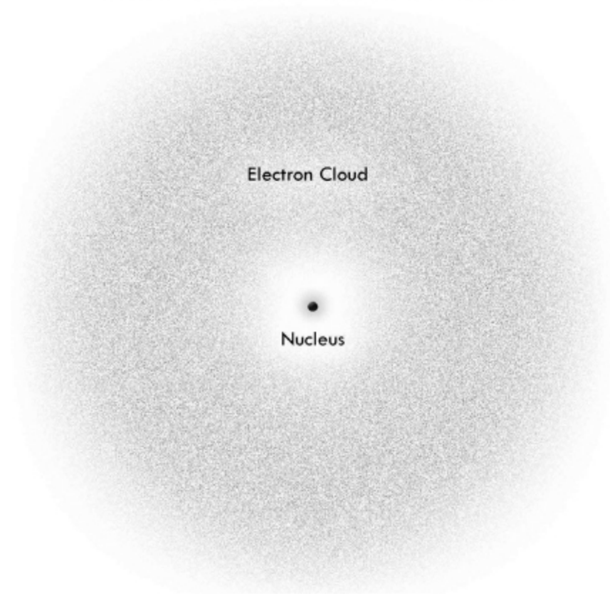
Figure 1B. The “new-school” quantum version of an atom with an electron cloud. The atom is 99.99999 percent energy and .00001 percent matter. It’s just about nothing, materially.
