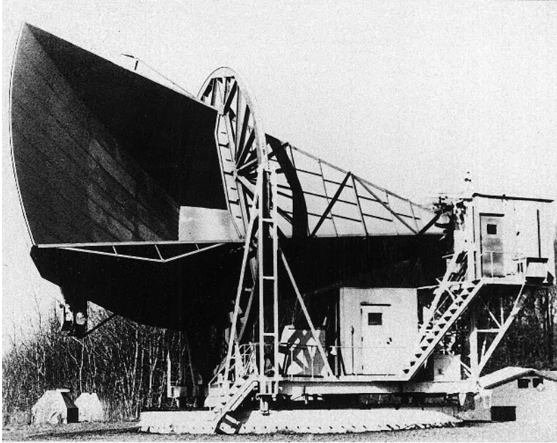
Figure 19.7. The 20-foot parabolic horn-shaped antenna of the Bell Telephone Laboratories at Holmdell, in New Jersey, used by Arno Penzias and Robert Wilson in their discovery of the cosmic microwave background radiation in 1965. (Courtesy of Robert Wilson. Copyright, 1978, with permission of Lucent Technologies.)
