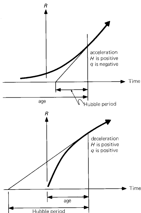
Figure 14.21. Expansion in accelerating and decelerating universes. Notice that in accelerating universes the age is greater than the Hubble period, and in decelerating universes the age is less than the Hubble period.
