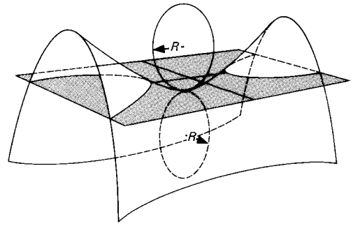
Figure 10.7. A saddle-shaped surface has negative curvature. Only the central region of the saddle is representative of uniform hyperbolic space; far from the central region, however, the surface is neither homogeneous nor isotropic. The radii R of curvature are on opposite sides of the surface, thus making the curvature ( K = -1/R^2 ) negative.
