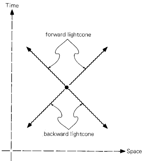
Figure 11.2. A lightcone at a point in spacetime. Light comes in from the past on the backward lightcone and goes out into the future on the forward lightcone.
