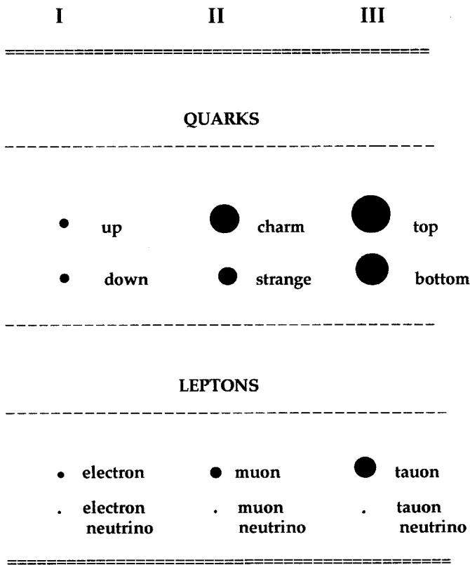
Figure 20.7. This shows the three lepton–quark families of the grand unified theory. Size indicates mass (or energy). Family I consists of the electron and its neutrino, and the up and down quarks of nuclear matter. The ordinary low-energy world around us is composed solely of these fundamental matter particles. Family II (the muon and its neutrino plus the charm and strange quarks), and family III (the tauon and its neutrino plus the top and bottom quarks) consist of particles that compose the worlds of high energy.
