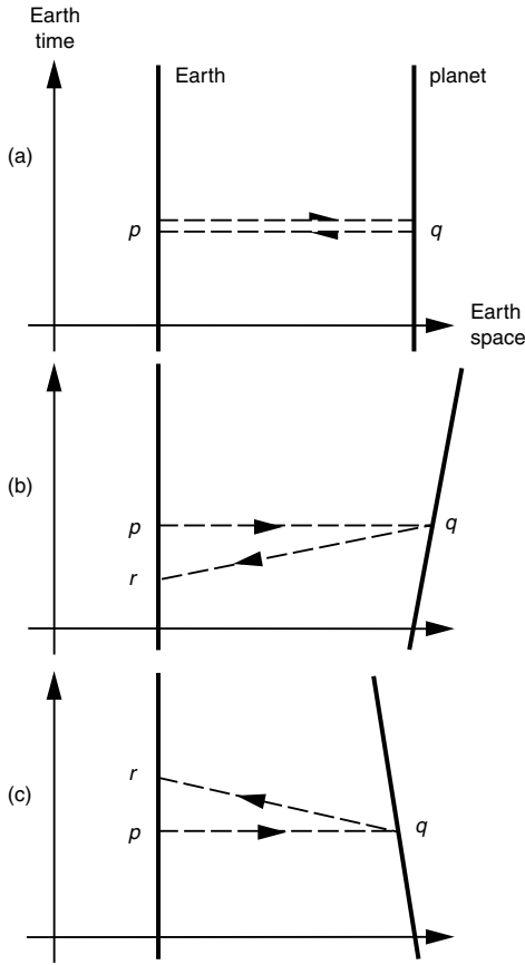
Figure 11.14. People on Earth and on a distant planet communicate with each other by M-rays (M for mystic) that travel at infinite speed. In (a) the distant planet is stationary relative to Earth. Signals sent from Earth at instant p arrive instantaneously in Earth time at the planet at instant q and their return is also instantaneous. In (b) the planet is shown moving away from Earth. Signals sent from Earth at instant p arrive at the planet at instant q , and the return signals travel instantaneously in the planet's time and arrive on Earth at instant r , which lies in Earth's past. In diagram (c) the distant planet is shown moving toward the Earth. Signals sent from Earth at instant p travel infinitely rapidly and arrive at the planet at instant q , and the return signals travel instantaneously in the planet's time and arrive on Earth at instant r , which lies in Earth's future. If M-rays existed, we could communicate directly with our descendants and ancestors by using distant mirrors moving away and toward the Earth.
