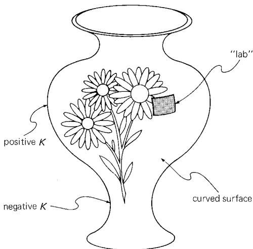
Figure 12.11. A thin and malleable piece of material, labeled “lab,” fits snugly on a curved surface. The variation of curvature within the lab is analogous to the variation of gravity (the tidal force) within a free-falling laboratory.
