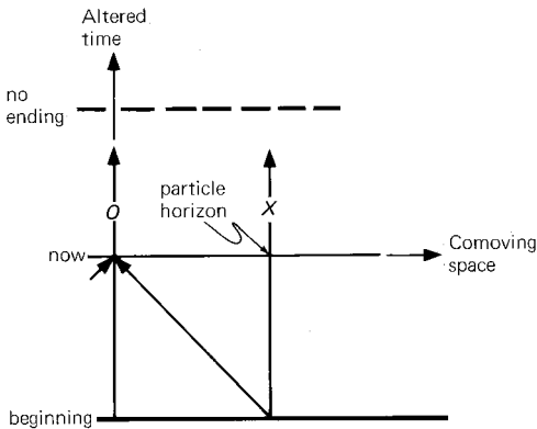
Figure 21.16. A conformal spacetime diagram in which altered time has a beginning but no ending. The particle horizon is at world line X, and no event horizon exists.
