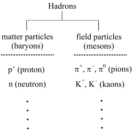
Figure 20.5. Hadrons are the strongly interacting particles. Like leptons they consist of matter particles (fermions) that are the baryons, and field particles (bosons) that are the mesons. The matter particles on the left comprise nucleons (neutrons and protons) and many short-lived particles (such as the lambdas, sigmas, xis, and omegas); the field particles on the right comprise mesons (such as the pions and kaons). Unlike the leptons, which are structureless and irreducible, the hadrons possess complex structure and are composed of quarks.
