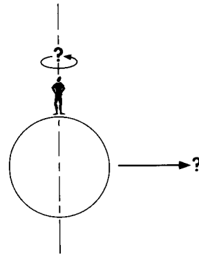
Figure 12.19. Berkeley's "solitary globe" in an otherwise empty universe. All forms of motion, uniform and accelerated, are unobservable and meaningless, according to Berkeley.
