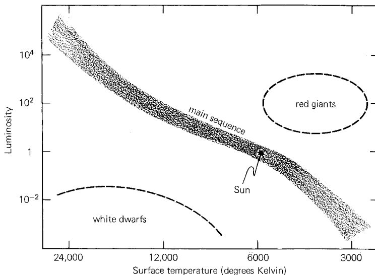
Figure 5.3. The Hertzsprung–Russell diagram in which the brightness (or luminosity) and the color (or surface temperature) of stars are plotted. The luminosity is expressed in units of the Sun's luminosity.
