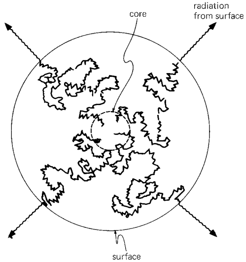
Figure 5.5. Radiation in a star is continually scattered by gas particles and slowly diffuses to the surface. In the Sun the energy generated in the central region takes about 20 million years to reach the surface.
