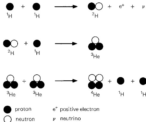
Figure 5.9. The fusion of four protons into one helium nucleus. First, two protons ( {}^1\text{H} + {}^1\text{H} ) combine to form a deuteron ( {}^2\text{H} ) consisting of one proton and one neutron, and a positive electron ( e^+ ) and a neutrino ( \nu ) are created by the reaction. This is a very slow process that takes about 10 billion years in the center of the Sun. Once formed, a deuteron quickly picks up an additional proton and becomes a helium-3 ( {}^3\text{He} ) nucleus. Two helium-3 nuclei then combine to produce one helium-4 ( {}^4\text{He} ) nucleus and two free protons. This conversion of four protons into one helium nucleus is the important proton chain of reactions. Competing reactions exist; for example, helium-3 combines with helium-4 to produce a beryllium-7 ( {}^7\text{Be} ) nucleus that by proton capture becomes two separate helium nuclei.
