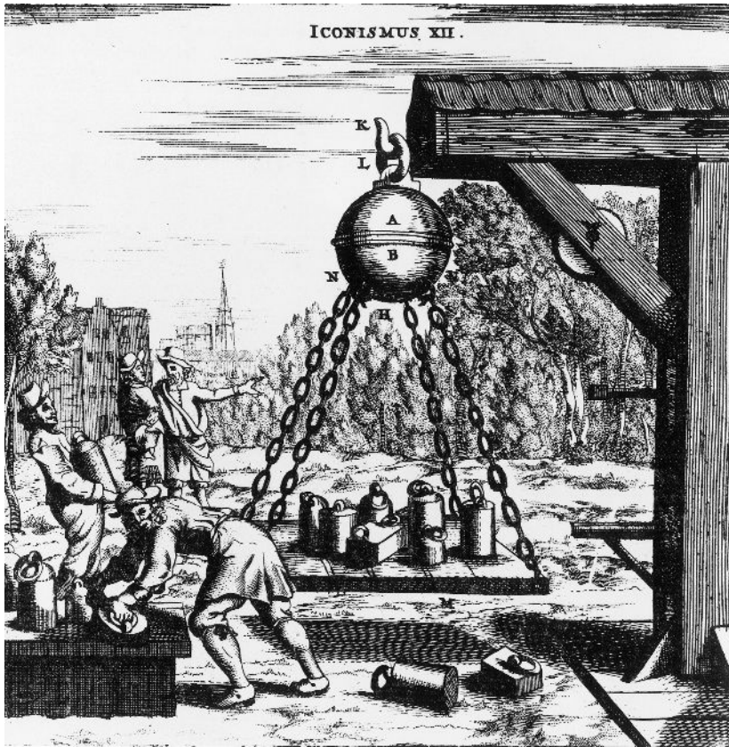
Figure 9.1. Otto von Guericke, mayor of Magdeburg, constructed in 1650 the first air pump and in subsequent years made spectacular demonstrations of the properties of the vacuum. He showed that sound does not propagate and candles do not burn in the absence of air. In the experiment shown in this illustration he measured the atmospheric pressure holding together the two halves of an evacuated sphere.
