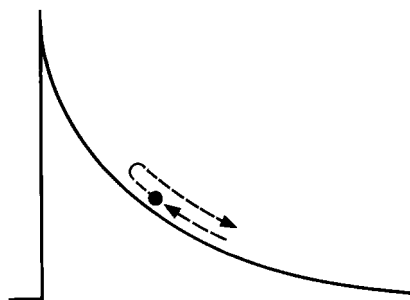
Figure 5.7. The electrical repulsion between two protons is like a hill. Two protons approach, and because of mutual repulsion each, in effect, climbs a hill. But normally they lack sufficient energy to reach the top, so they fall back and go off in new directions.
