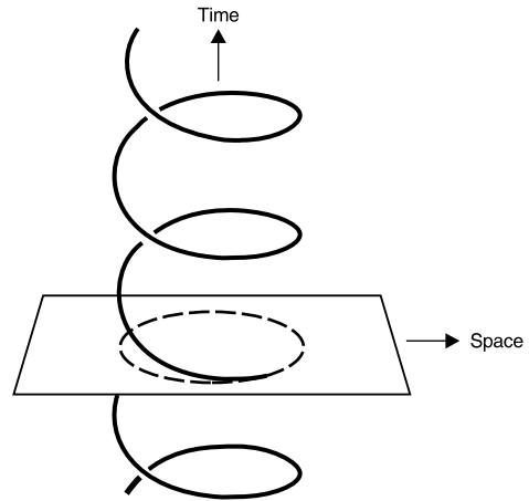
Figure 9.7. Charles Hinton's illustration of a world line (which he called a filamentary atom) of a particle in circular motion. The world line is a helix, and as time advances the particle describes a circle in space.
