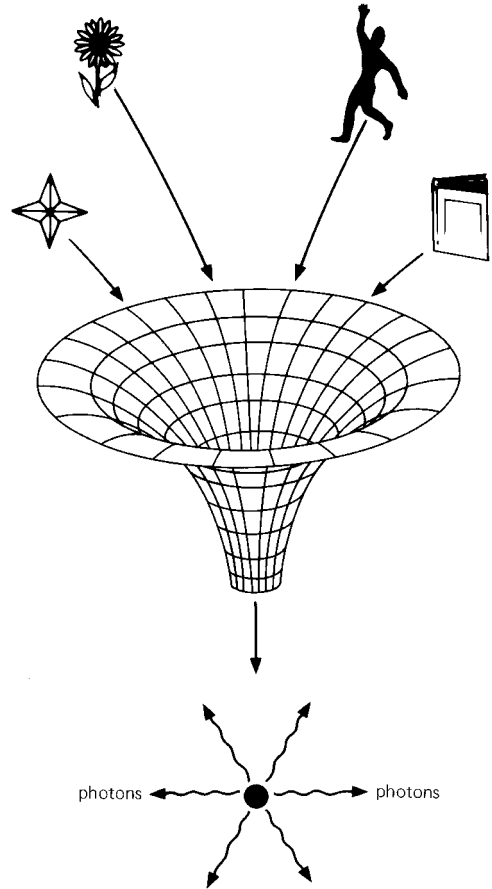
Figure 13.19. A black hole is a sink of lost information. It is also a machine that generates entropy.
