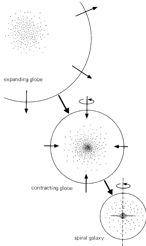
Figure 6.12. This figure shows one possible way in which a spiral galaxy might form. The expanding universe, already hundreds of millions of years old, has fragmented into large globes of gas. At first, each globe continues to expand, but slower than the universe, then later it stops expanding and begins to collapse. Population II stars in large numbers form in the central region. Gas from the outer regions of the globe falls inward and forms a rotating disk in which population I stars are slowly born.
