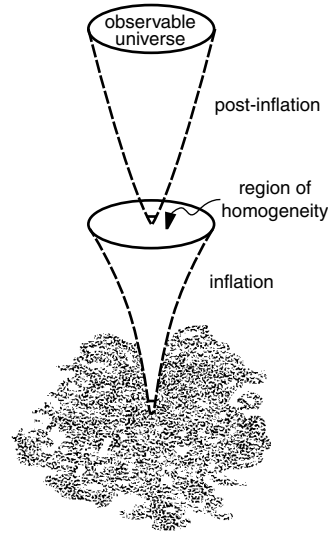
Figure 22.5. Tiny homogenized regions in the pre-inflationary era are the size of a Hubble sphere of radius 10^{-26} centimeters. Such regions rapidly expand in the inflationary era and become enormously large. In the post-inflation era these enormous regions continue to expand with positive deceleration. A small part of one of these enormous expanding regions, initially about 1 centimeter radius, is now our present observable universe of 10 billion light years radius.
