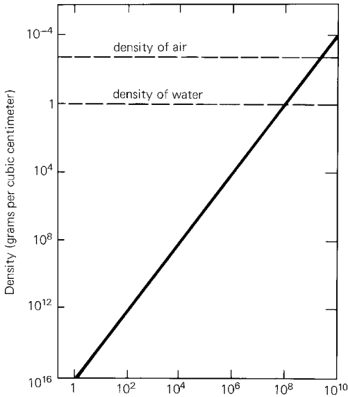
Figure 13.14. The average density of a black hole decreases as mass increases. A black hole 100 million solar masses has an average density equal to that of water, and a black hole of 3000 million solar masses has an average density equal to that of air at sea level.
