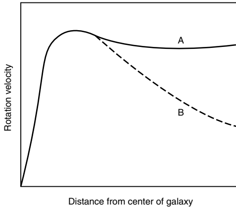
Figure 19.3. A schematic rotation curve of a spiral galaxy – such as the Galaxy – showing how the rotation velocity varies with radius. Beyond 30 000 light years the rotation velocity tends to be flat, as shown by curve A, indicating that considerable nonluminous mass exists in the outer regions of the Galaxy. If no mass existed beyond 30 000 light years, the rotation velocity would fall off in the way shown by the dashed curve B.
