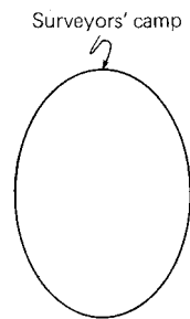
Figure 7.2. A finite unbounded surface that is egg-shaped. The Surveyors' camp is at one end of the egg.
