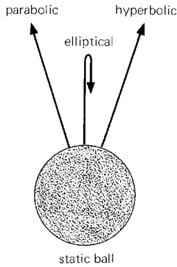
Figure 16.3. Particles move away radially from the surface of a gravitating sphere. The initial velocity determines whether the orbit is parabolic, elliptical, or hyperbolic.
