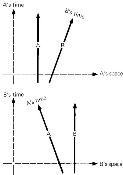
Figure 11.4. We can display a spacetime diagram so that either A's space is shown perpendicular to A's world line or B's space is shown perpendicular to B's world line, but we cannot show simultaneously in a diagram the fact that both spaces are perpendicular to their world lines. This is because the geometry of spacetime is unlike the geometry of a blackboard or a sheet of paper.
