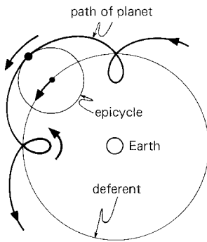
Figure 2.5. The motion of the planets according to the epicyclic theory. A planet revolves around on a small circle (an epicycle) whose center moves around on a large circle (the deferent) that has the Earth at its center of the universe. The planet is thus seen to move backward and forward, and the backward (retrograde) motion occurs when the planet is closer to Earth and appears brighter, in agreement with observation.
