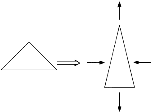
Figure 14.6. Shear only: triangles change their shape but not their area and orientation.
