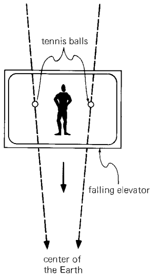
Figure 12.9. Two tennis balls float, as shown, in a free-falling elevator. As the elevator plunges toward the center of the Earth at an accelerating rate, the tennis balls move toward each other at an accelerating rate. To an observer in the elevator it seems that a force exists that acts on the two balls. This force, which is the result of the nonuniformity of gravity, is the tidal force.
