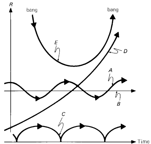
Figure 18.15. Universes in tension, where pressure is P = (\gamma - 1)\rho c^2 , \rho is the mass density, and \gamma is a constant. (A) A closed, oscillating universe in which 0 < \gamma < 2/3 ; (B) a closed, static, stable universe in which 0 < \gamma < 2/3 ; (C) a closed, constant-density, oscillating universe in which \gamma = 0 ; (D) a flat, constant-density, steady-state universe in which \gamma = 0 ; and (E) all open and closed universes in which \gamma < 0 , which expand and become not whimpers but big bangs.
