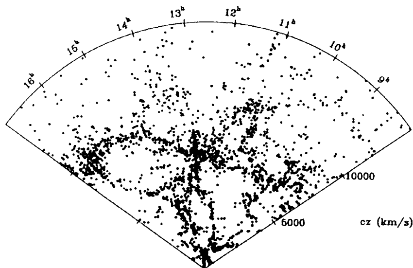
Figure 19.10. Center for Astrophysics redshift survey. This map contains 2529 galaxies of apparent magnitude m less than 15.6 in a slice of the north galactic cap between declination 26.5 and 44.5 degrees, displayed in right ascension. The radial coordinate is velocity in kilometers per second obtained from multiplying redshift by the speed of light. (Courtesy of John Huchra and Margaret Geller, with permission of the Harvard-Smithsonian Institute.)
