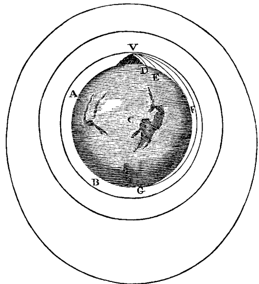
Figure 3.11. "The Stone that put the Stars to Flight" ( The Rubáiyát ). Newton wrote: "For a stone ... the greater the velocity with which it is projected, the farther it goes before it falls to Earth ... till at last, exceeding the limits of the Earth it will pass into space." Illustration and quotation from The System of the World by Isaac Newton.
