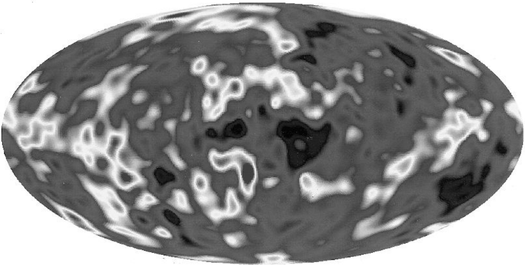
Figure 19.9. A full sky simulation of an anisotropy map based on four years of observations made with the Cosmic Background Explorer. The temperature difference between the black and white regions is 10^{-4} kelvin. (Reproduced courtesy of Gary Hinshaw at NASA, Goddard Space Flight Center.)
