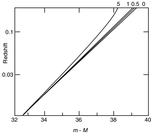
Figure 19.11. A set of curves according to Equation [19.29], showing redshift plotted against the distance modulus m-M for q = 5, 1, 0.5, 0 , assuming that h = 1 . The curvature has no effect on the shape of these curves; similarly with Figure 19.12.
