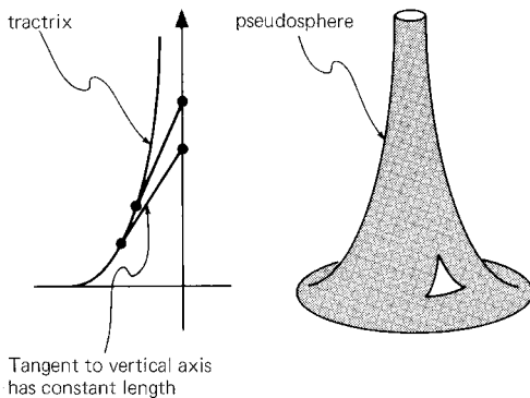
Figure 10.6. The surface of a pseudosphere has hyperbolic geometry of negative curvature. The sum of the interior angles of a triangle is less than two right angles. The curvature of the surface, however, is not homogeneous (the same at all places).
