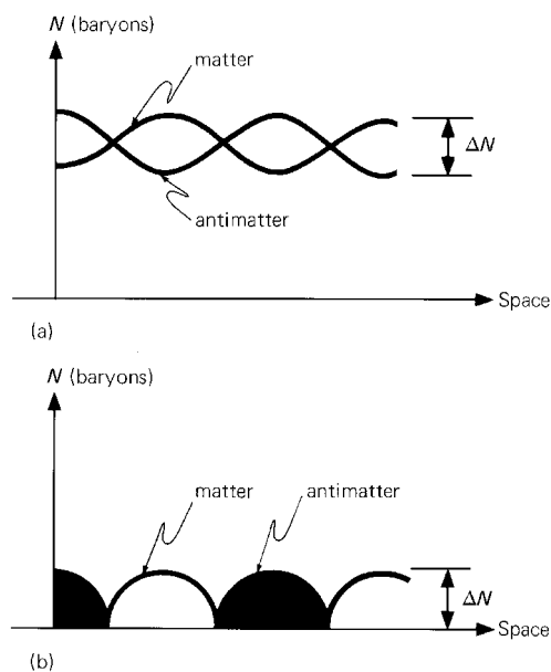
Figure 20.9. In (a) the densities of matter and antimatter vary relative to each other, and their average densities are supposed equal. After annihilation, only their difference survives, as shown in (b), and isolated regions exist of matter and antimatter.
