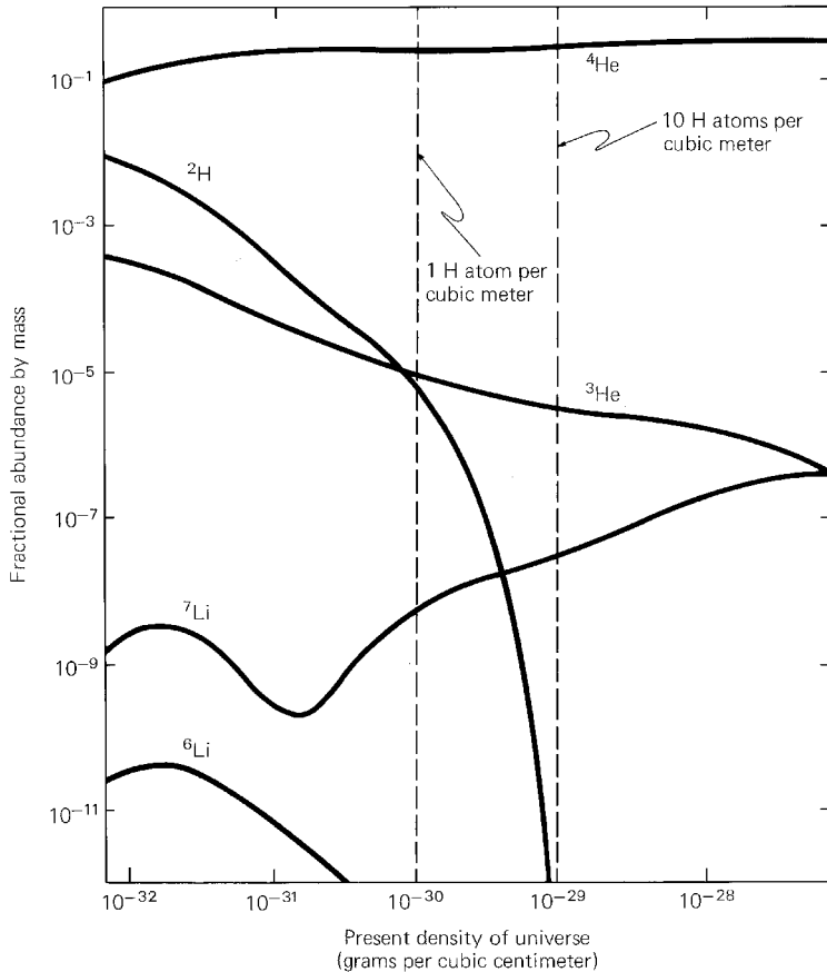
Figure 19.6. The abundances of deuterium ( ^2\text{H} ), helium ( ^3\text{He} and ^4\text{He} ), and lithium ( ^6\text{Li} and ^7\text{Li} ) produced in the first 200 seconds of the early universe. The curves show how the mass fractions of these elements relate to the present-day average density of baryonic matter in the universe. Notice how the deuterium abundance is sensitive to the matter density: the more dense the matter, the more frequently deuterium nuclei collide with one another in the early universe and combine to form helium nuclei. Adapted from David Schramm and Robert Wagoner, "What can deuterium tell us?: Physics Today (1974).
