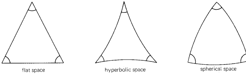
Figure 10.3. Triangles in flat, hyperbolic, and spherical spaces.
