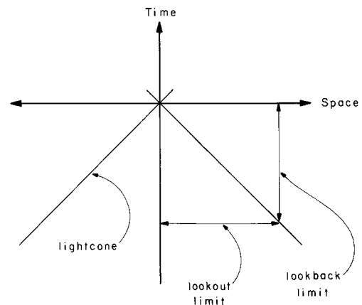
Figure 24.8. Spacetime diagram showing the lookout limit in space and the lookback limit in time.
