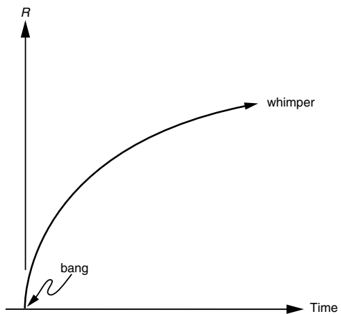
Figure 16.7. A Friedmann universe of zero curvature ( k = 0 ), also known as the Einstein–de Sitter universe.
