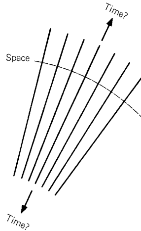
Figure 9.11. Spacetime picture of diverging (converging) world lines in an expanding (contracting) universe. Does this picture fix the direction of time?
