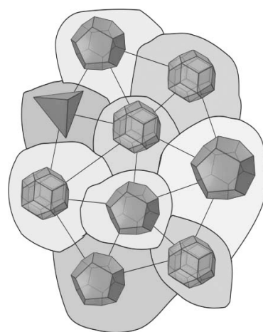
Representation of the web of elementary grains of space (or spin network).
